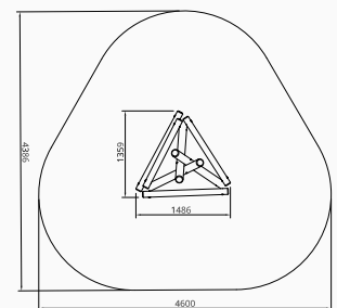
Plan elevation
