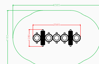
Plan elevation
