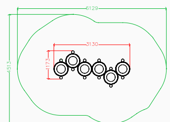
Plan elevation
