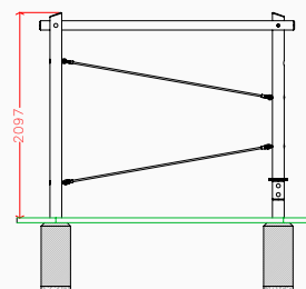
Plan elevation
