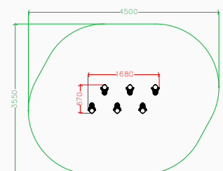
Plan elevation
