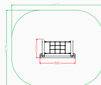
Plan elevation
