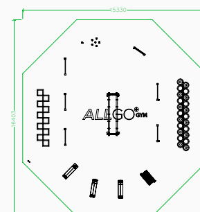
Plan elevation
