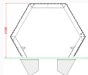
Side elevation
