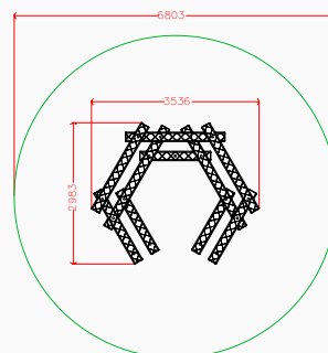
Plan elevation
