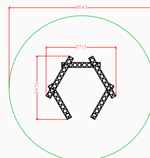
Plan elevation
