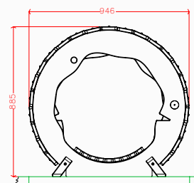
Plan elevation
