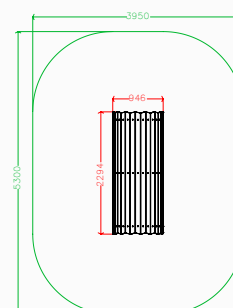
Plan elevation
