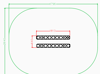
Plan elevation
