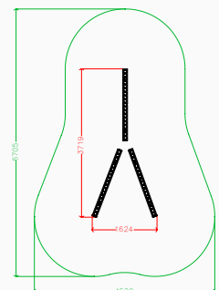
Plan elevation
