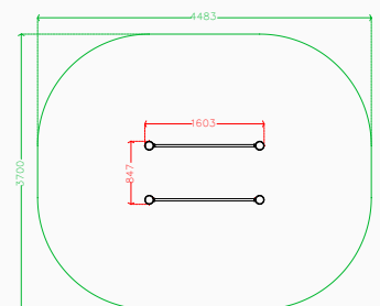
Plan elevation
