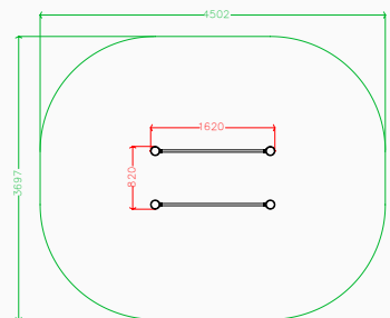
Plan elevation
