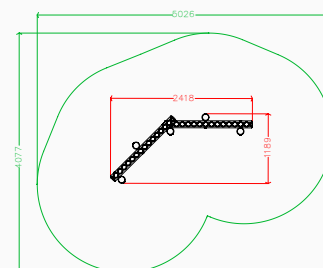
Plan elevation
