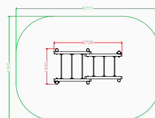
Plan elevation
