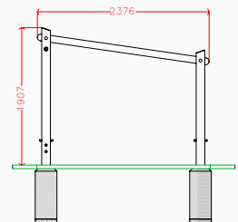
Side elevation
