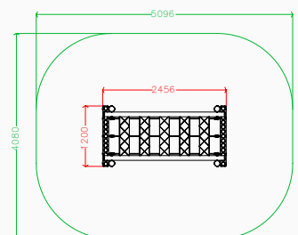
Plan elevation
