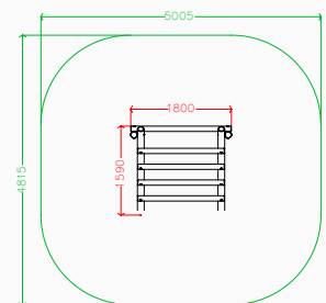
Plan elevation
