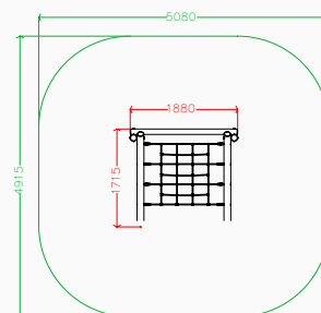
Plan elevation
