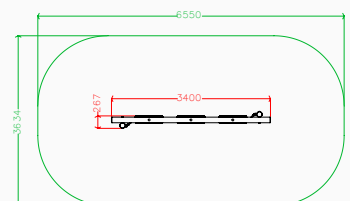
Plan elevation
