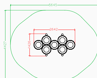
Plan elevation
