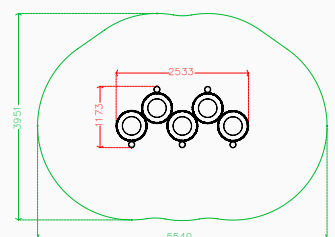
Plan elevation
