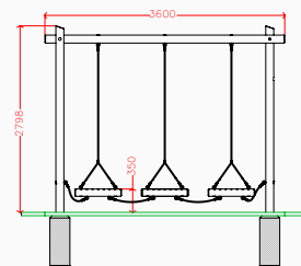
Side elevation
