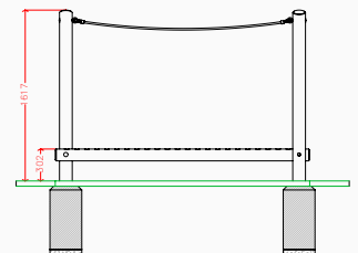
Side elevation
