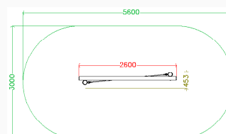
Plan elevation
