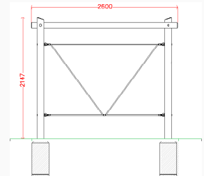
Side elevation
