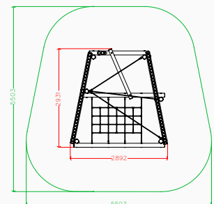
Plan elevation
