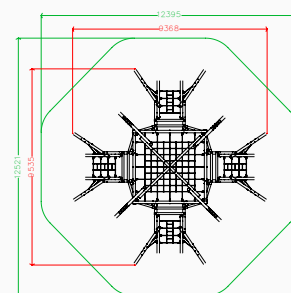
Plan elevation
