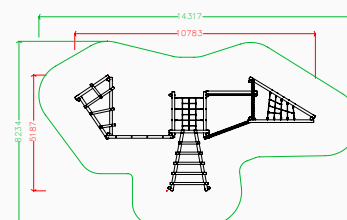
Plan elevation
