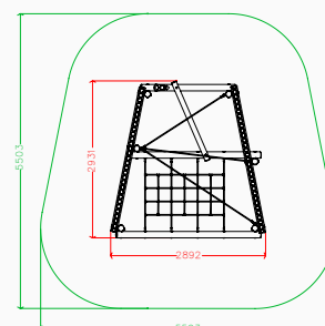
Plan elevation
