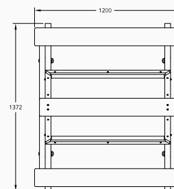
Plan elevation
