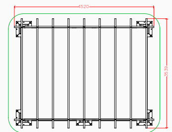
Plan elevation
