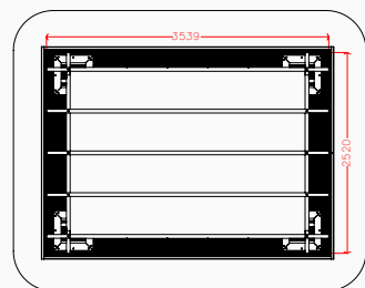
Plan elevation
