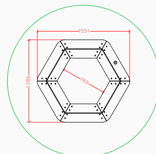
Plan elevation
