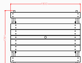
Plan elevation
