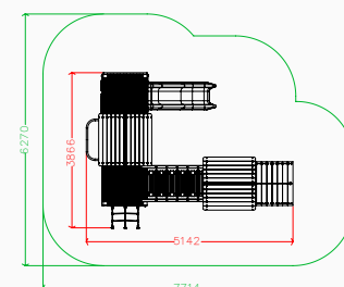
Plan elevation
