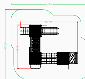
Plan elevation
