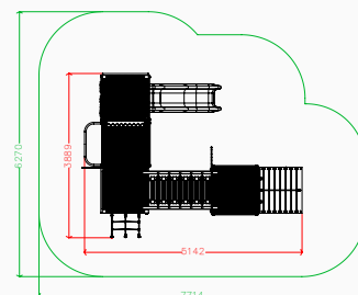
Plan elevation
