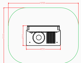
Plan elevation
