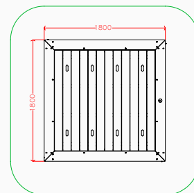
Plan elevation
