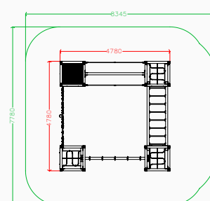
Plan elevation
