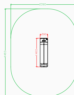
Plan elevation
