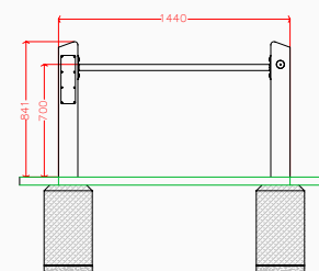
Plan elevation
